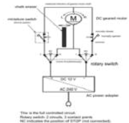
Figure 2: Circuit Diagram
